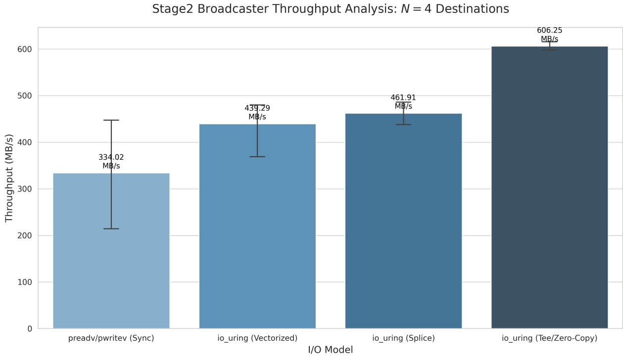
Figure 2: Performance characterization.
